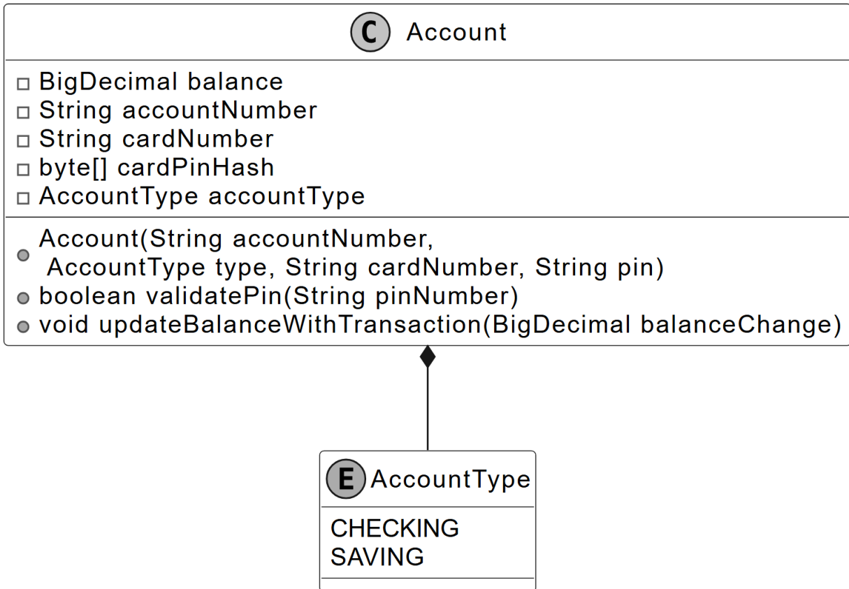
Account class and AccountType enum
