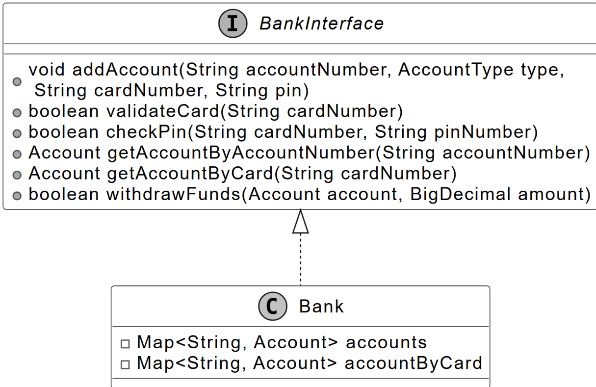
BankInterface interface and concrete class
