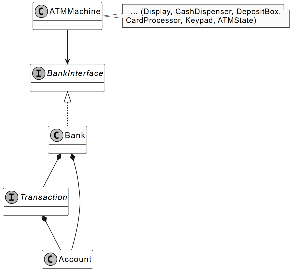
Summarized Class Diagram of ATM System
